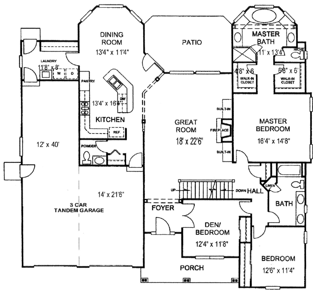
MAIN LEVEL
